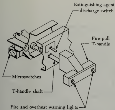
FIGURE 9-11. Fire-pull T-handle switch.
